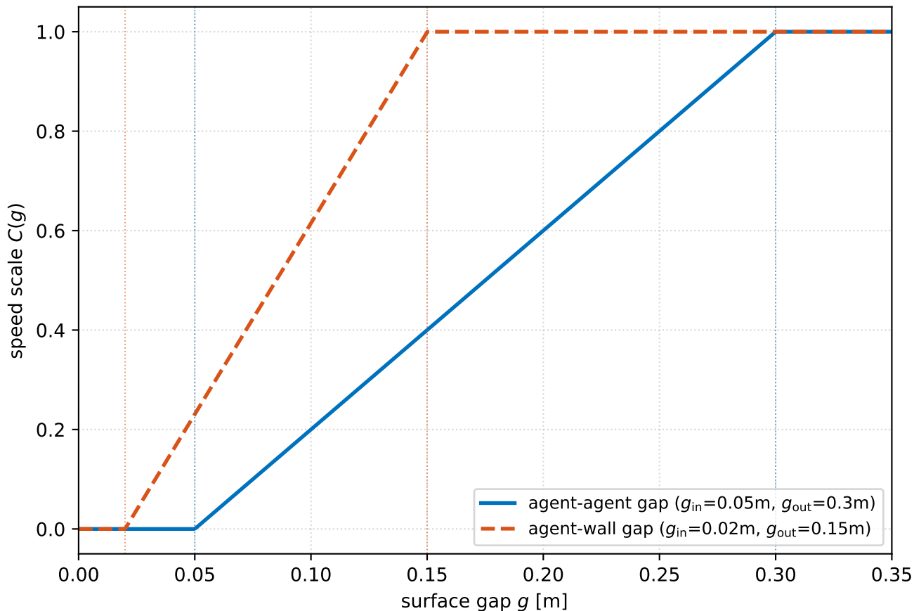
Safety-clamp forward-speed scale function C(g)
