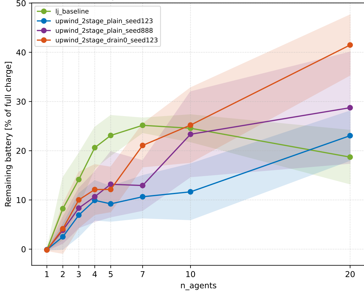
Battery vs. swarm size (mean \pm 1 std, 30 seeds)
