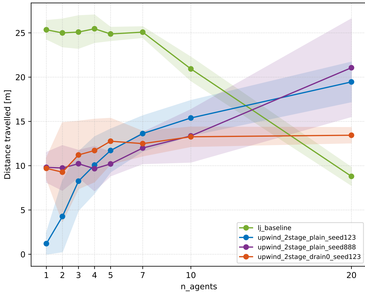
Distance vs. swarm size (mean \pm 1 std, 30 seeds)
