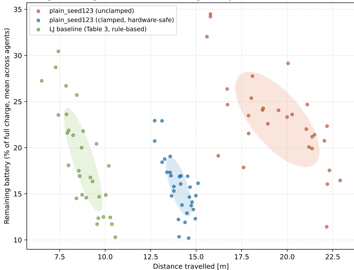
Fig. 5a analog -- distance vs. remaining battery (30 runs/condition, n=20)
