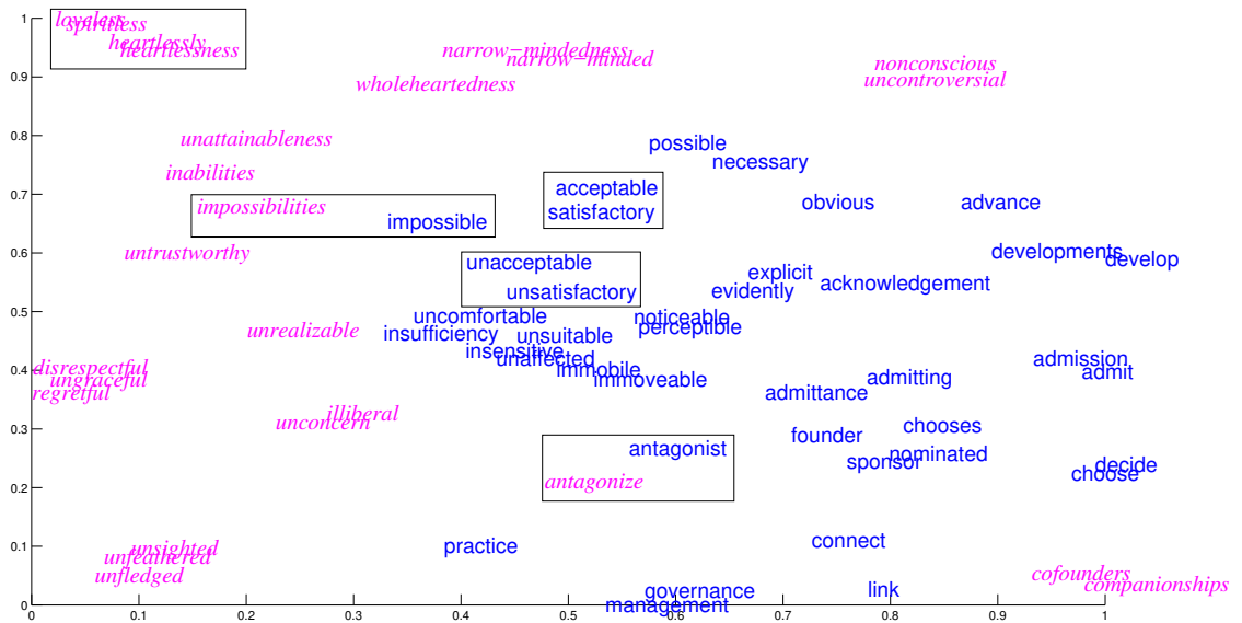
Figure 5.4: Barnes-Hut-SNE visualization of source word representations – shown are sample words from the Rare Word dataset. I differentiate two types of embeddings: frequent words in which encoder embeddings are looked up directly and rare words where I build representations from characters. Boxes highlight examples that I will discuss in the text. I use the hybrid model ( l ) in this visualization.
