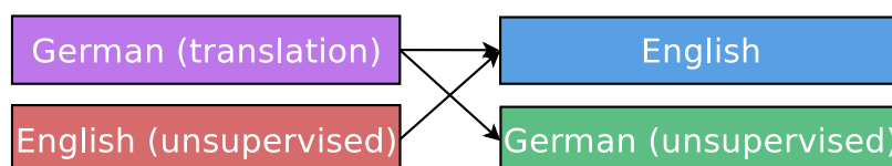
Figure 6.4: Many-to-many setting – multiple encoders, multiple decoders. I consider this scheme in a limited context of machine translation to utilize the large monolingual corpora in both the source and the target languages. Here, I consider a single translation task and two unsupervised autoencoder tasks.
