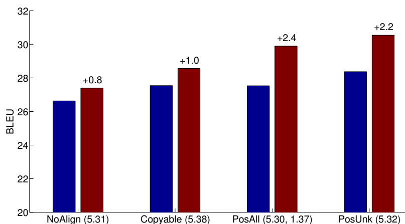
Figure 3.6: Rare word models – translation performance of 6-layer LSTMs: a model that uses no alignment ( NoAlign ) and the other rare word models ( Copyable , PosAll , PosUnk ). For each model, I show results before ( left ) and after ( right ) the rare word translation as well as the perplexity (in parentheses). For PosAll , I report the perplexities of predicting the words and the positions.
