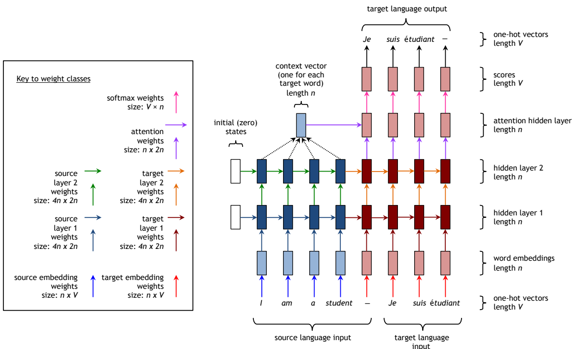
Figure 6.5: NMT architecture. This example has two layers, but my system has four. The different weight classes are indicated by arrows of different color (the black arrows in the top right represent simply choosing the highest-scoring word, and thus require no parameters). Best viewed in color.
