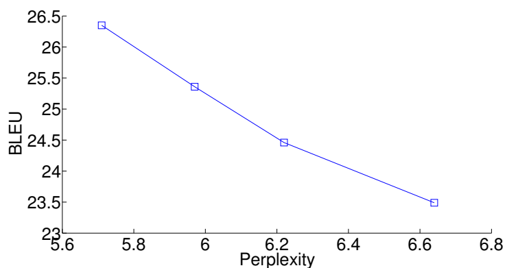
Figure 3.8: Perplexity vs. BLEU – I show the correlation by evaluating an LSTM model with 4 layers at various stages of training.
