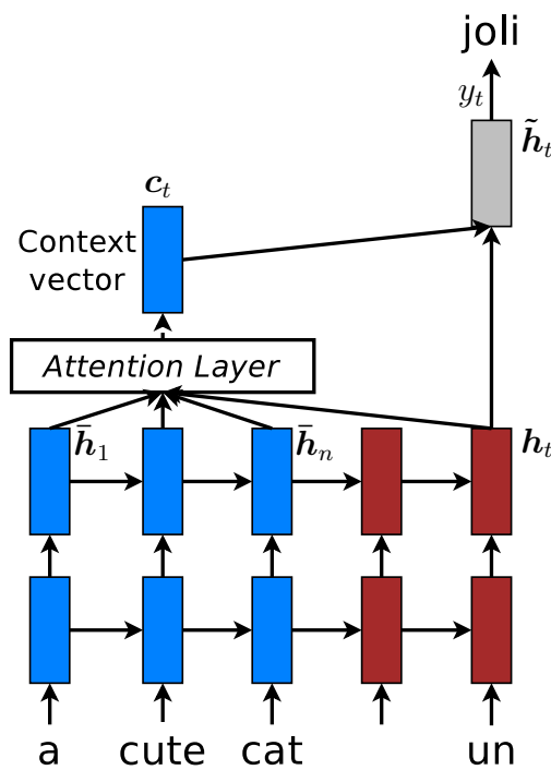
Figure 5.2: Attention mechanism – shown are the two steps of the attention mechanism I described in Chapter 4 (Luong et al., 2015b): first, compute a context vector c_t based on the current target hidden state h_t and all the source hidden states [\bar{h}_1, \dots, \bar{h}_n] ; second, use the context vector as an additional input to derive the attentional vector \tilde{h}_t .
