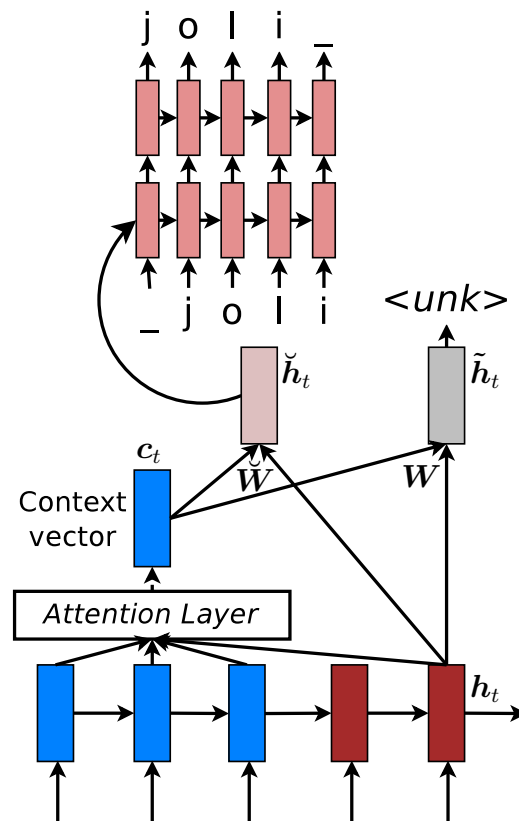
Figure 5.3: Separate-path Target Generation – two separate attentional vectors are created: \tilde{h}_t for predicting target words and \check{h}_t to seed the target-side character model.
