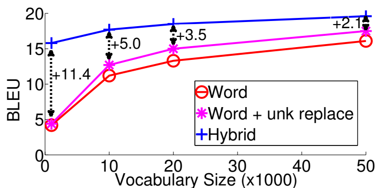
Figure 5.4: Vocabulary size effect – shown are the performances of different systems as I vary their vocabulary sizes. I highlight the improvements obtained by my hybrid models over word-based systems which already handle unknown words.
