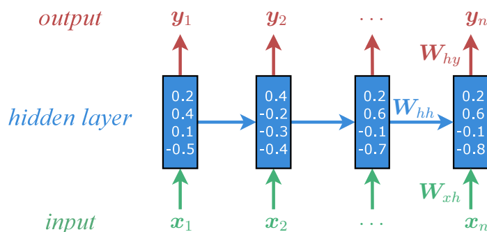
Figure 2.2: Recurrent neural networks – example of a recurrent neural network that processes an input sequence \mathbf{x}_1, \mathbf{x}_2, \dots, \mathbf{x}_n to build up hidden representations as each input is consumed and produces an output sequence \mathbf{y}_1, \mathbf{y}_2, \dots, \mathbf{y}_n . The input \mathbf{W}_{xh} , recurrent \mathbf{W}_{hh} , and output \mathbf{W}_{hy} weights are shared across timesteps.
