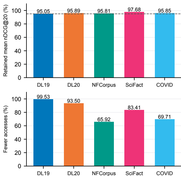
Fig. 3. Held-out mean quality retention and access reduction relative to exact Top-20 after 95% budget calibration. The dashed line marks the calibration target.
