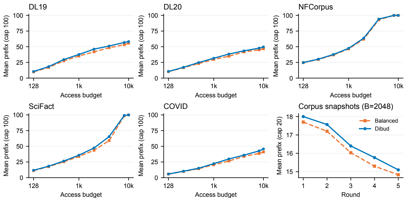
Fig. 2. Certified output under equal budgets. Static panels cap output at 100; the snapshot panel uses a cap of 20 and B = 2048 . All plotted budget endpoints are observed.
