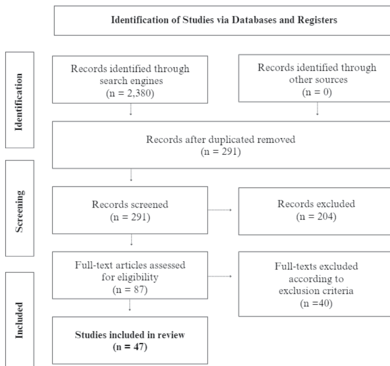
Fig. 4 PRISMA flow diagram
