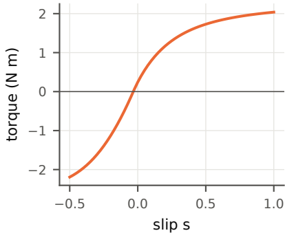
single wheel, nominal silica sand parameters, 12 kg rover
