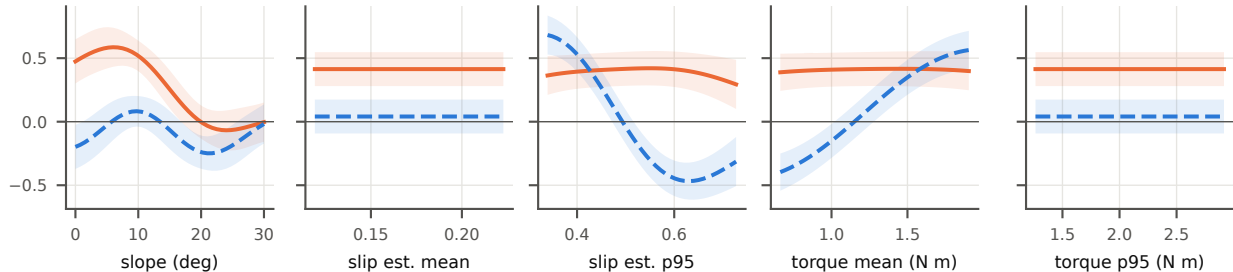
Stage C residual: each input swept over its training range, other inputs at the mean of that phase type
