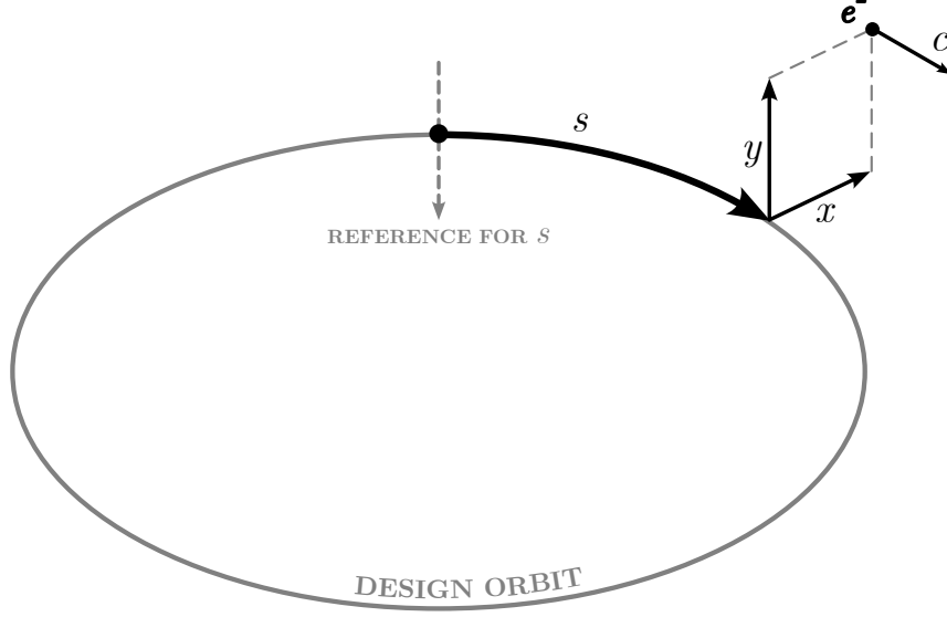
Figure 2.1: Coordinates for describing the electron trajectories.
