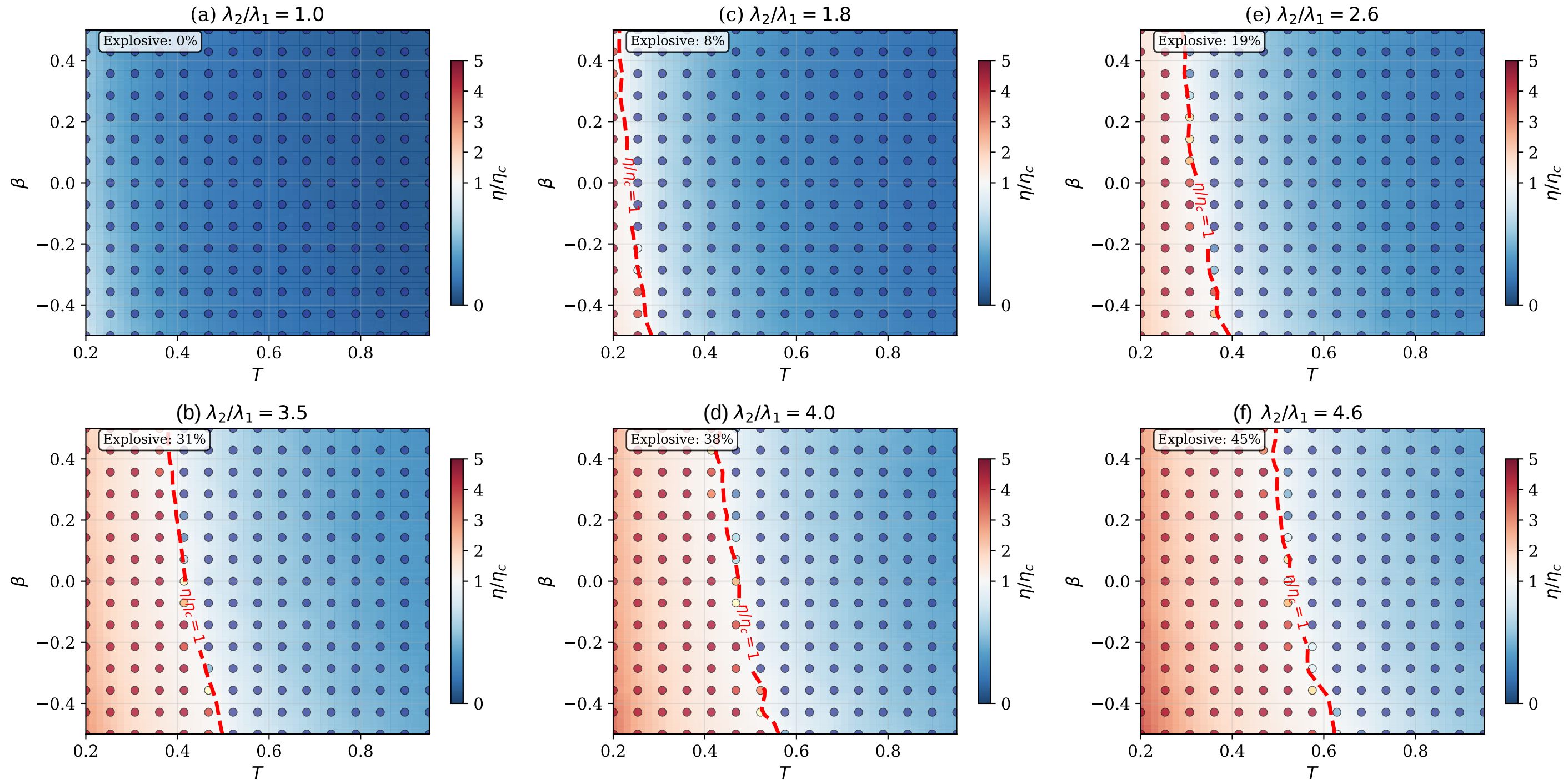
Figure 1: Phase diagram for SIS dynamics
