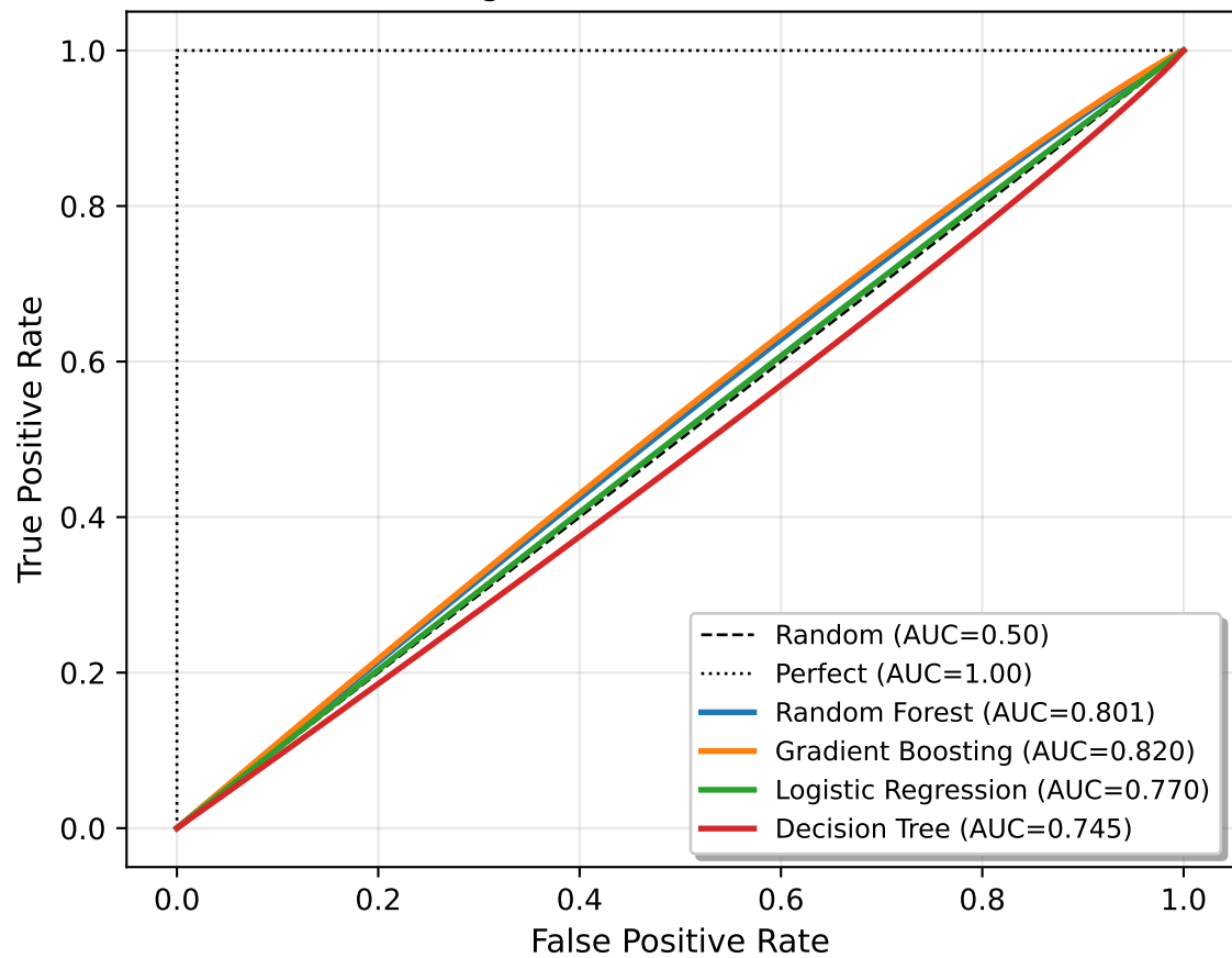
(b) GHALogs (GitHub Actions, 75.7K builds)
