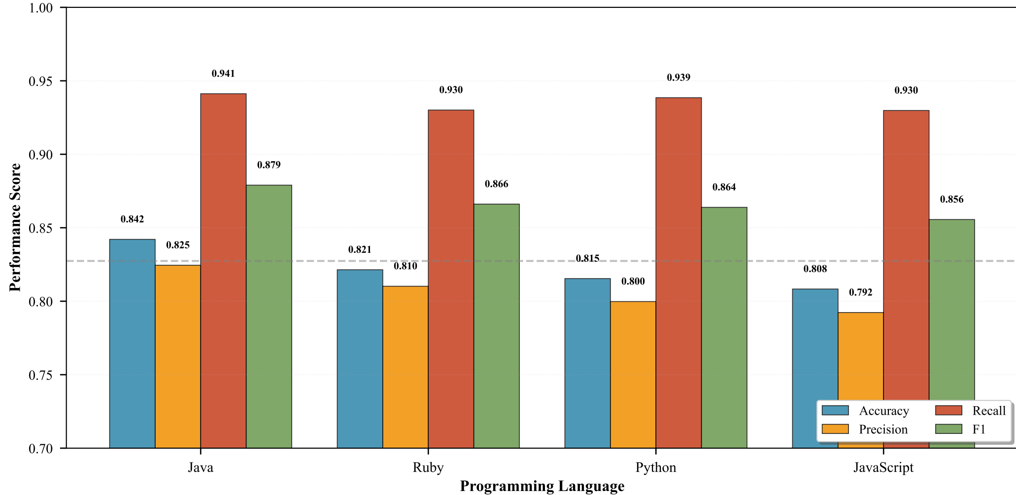
Cross-Language Build Prediction Performance (Random Forest Model, 20,000 Test Builds)
