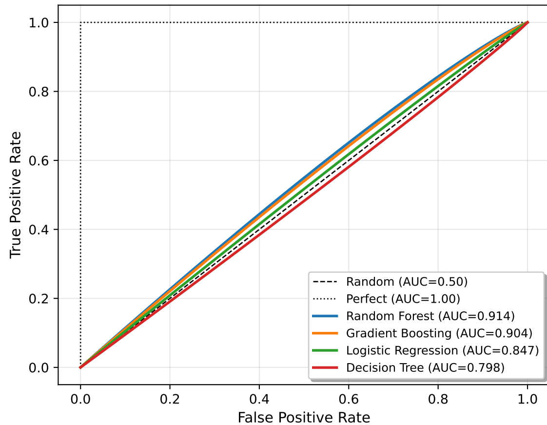
(a) TravisTorrent (Travis CI, 100K builds)
