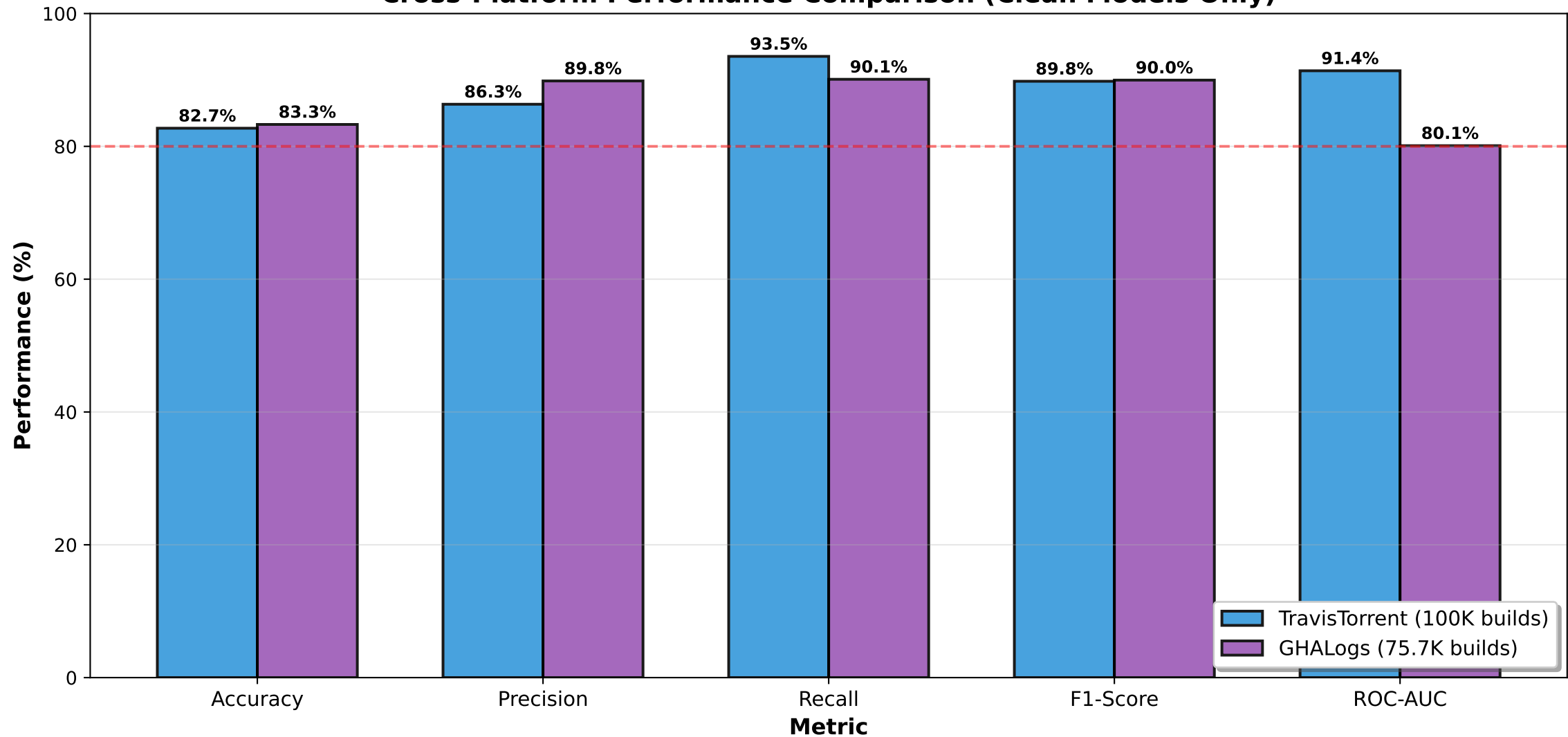
Cross-Platform Performance Comparison (Clean Models Only)
