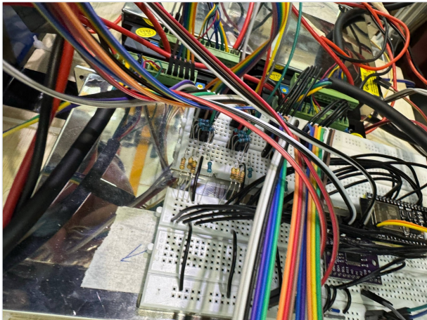
Level-shift circuit used in the drive test
