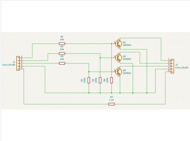
Level-shifter schematic (one motor)
