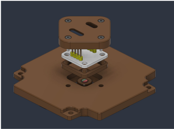
Modified motor cover + AS5600 (exploded CAD)
