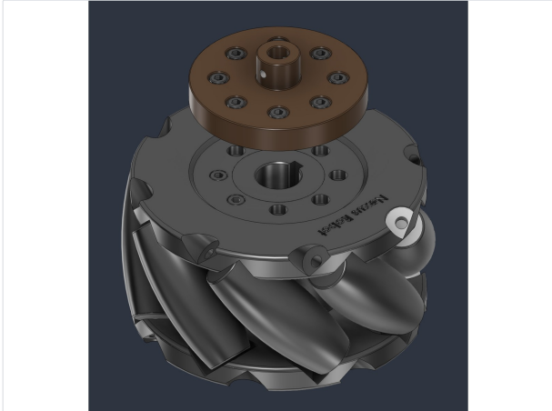
Wheel-hub adapter, mecanum wheel (CAD)
