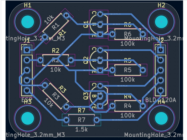
Level-shifter PCB layout (one motor)
