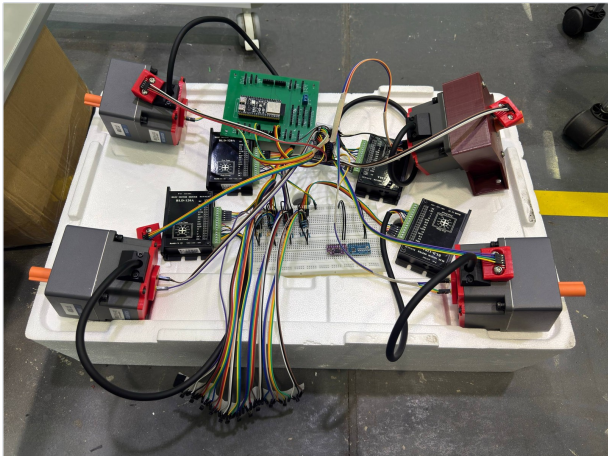
Base electronics, assembled (pre-mounting)
