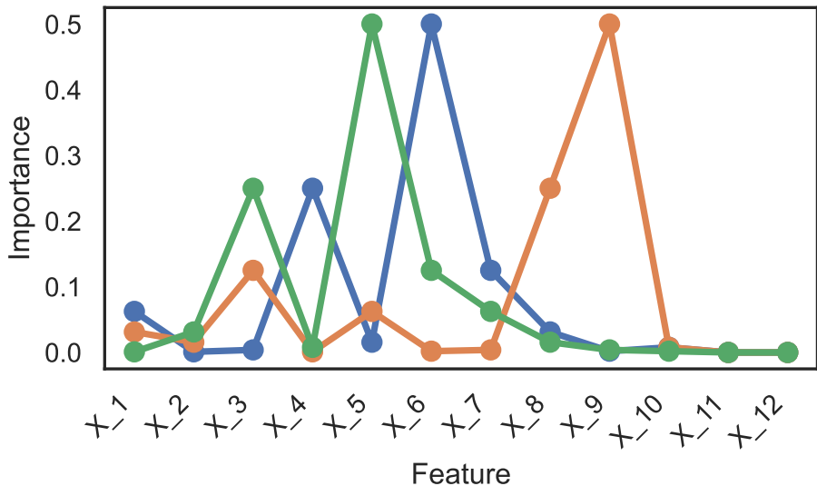
Gini Importance of Three Predictively Equivalent Trees
