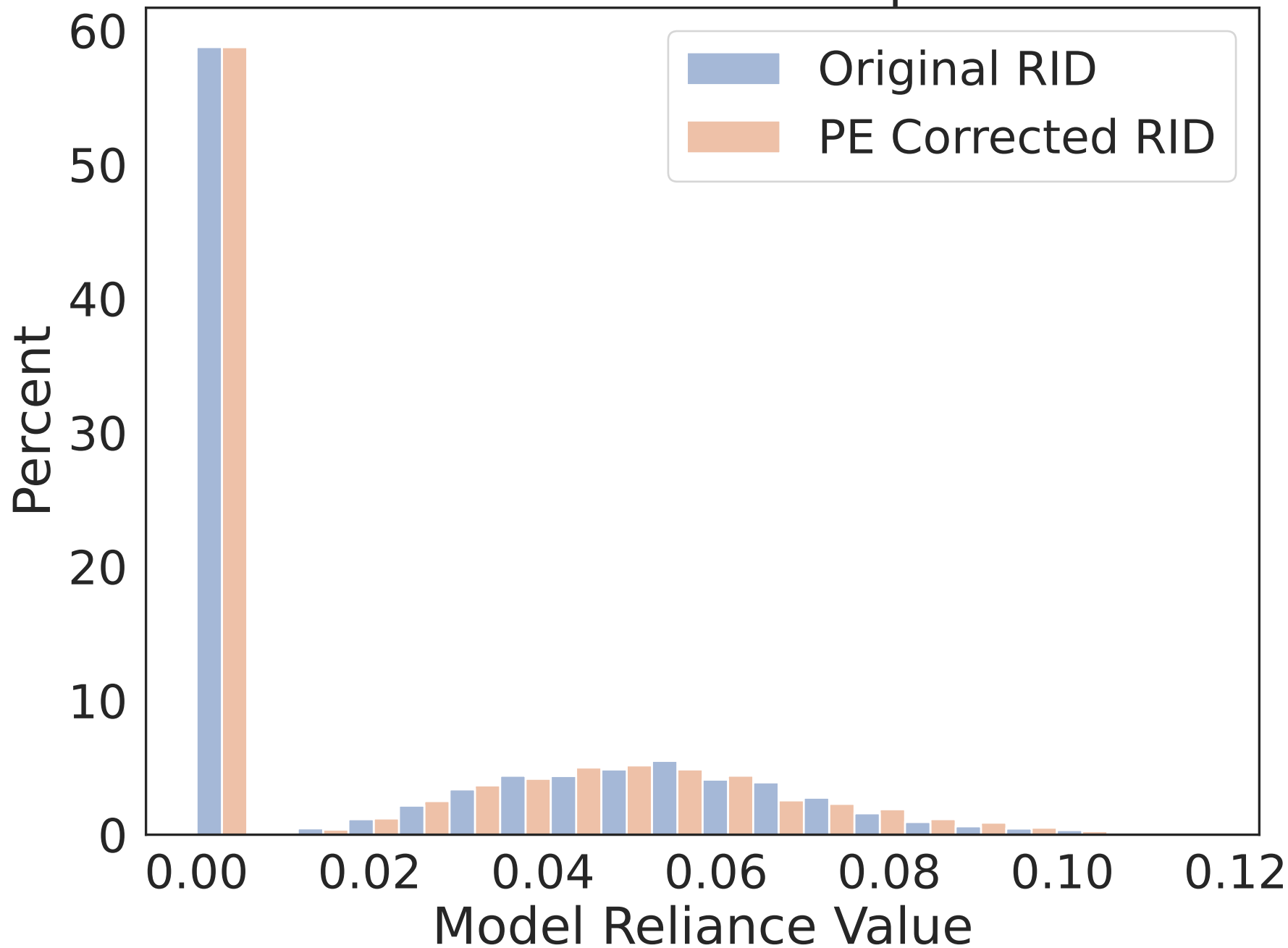
RID Distribution of 0 Importance
