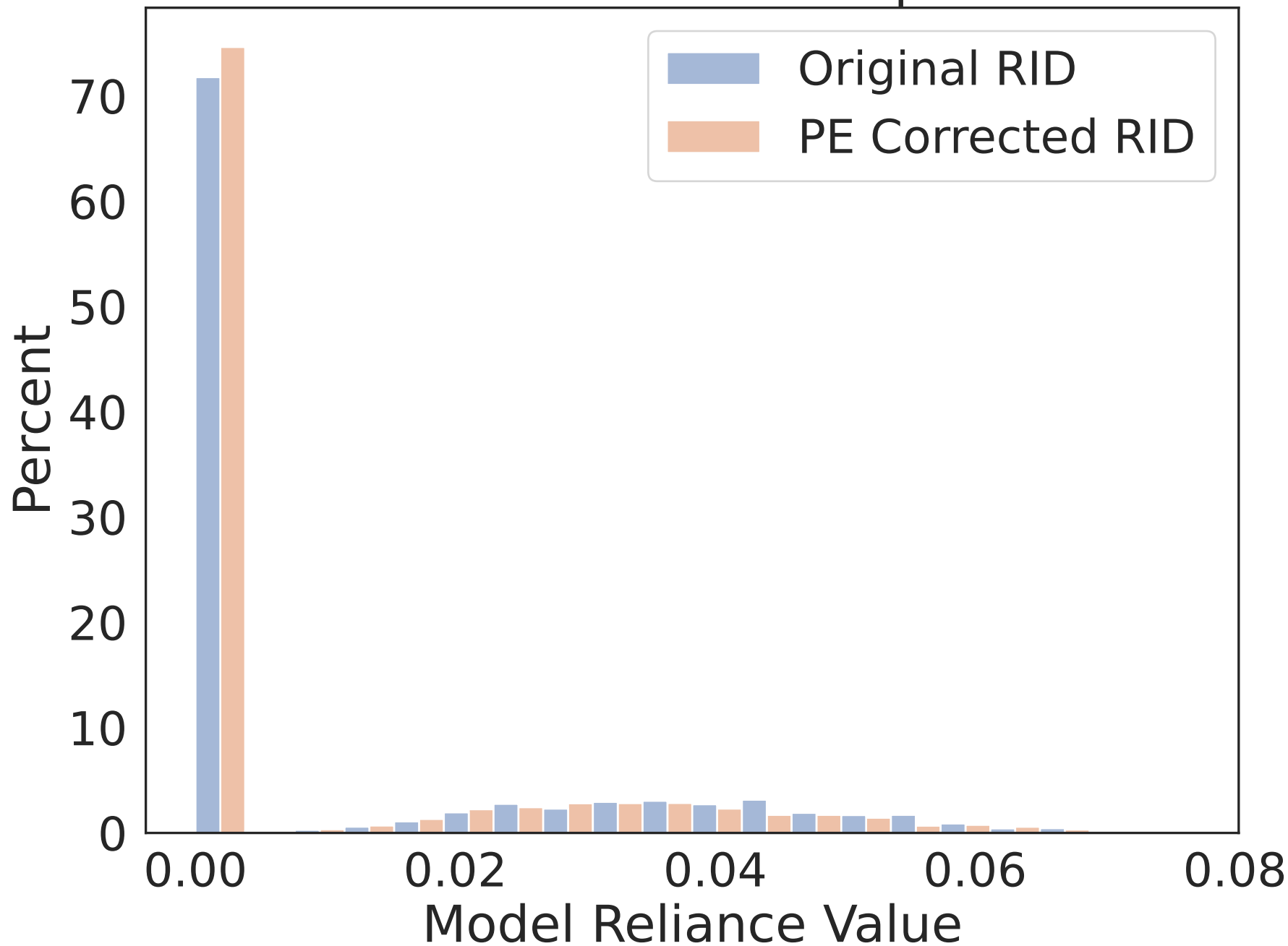
RID Distribution of 15 Importance
