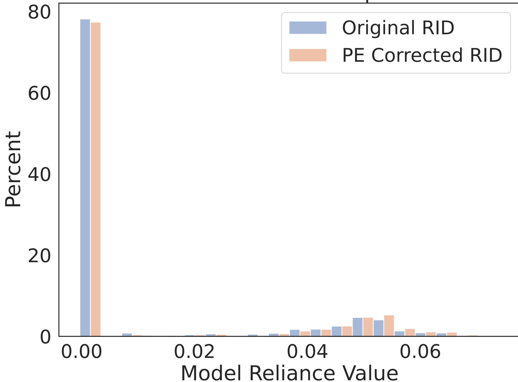
RID Distribution of 5 Importance
