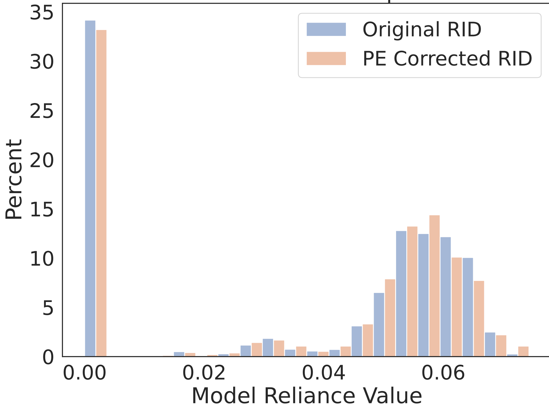
RID Distribution of 6 Importance
