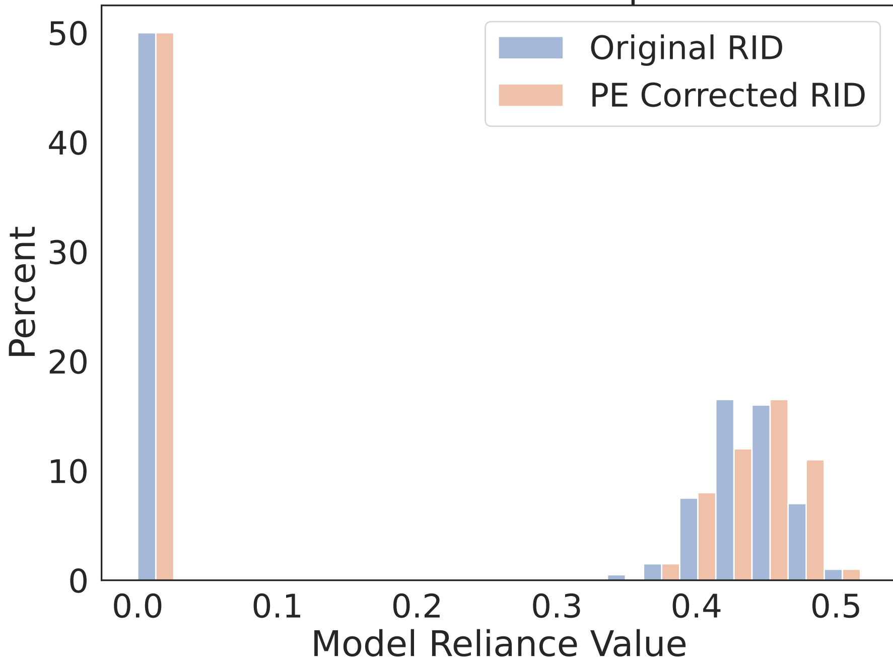
RID Distribution of 1 Importance
