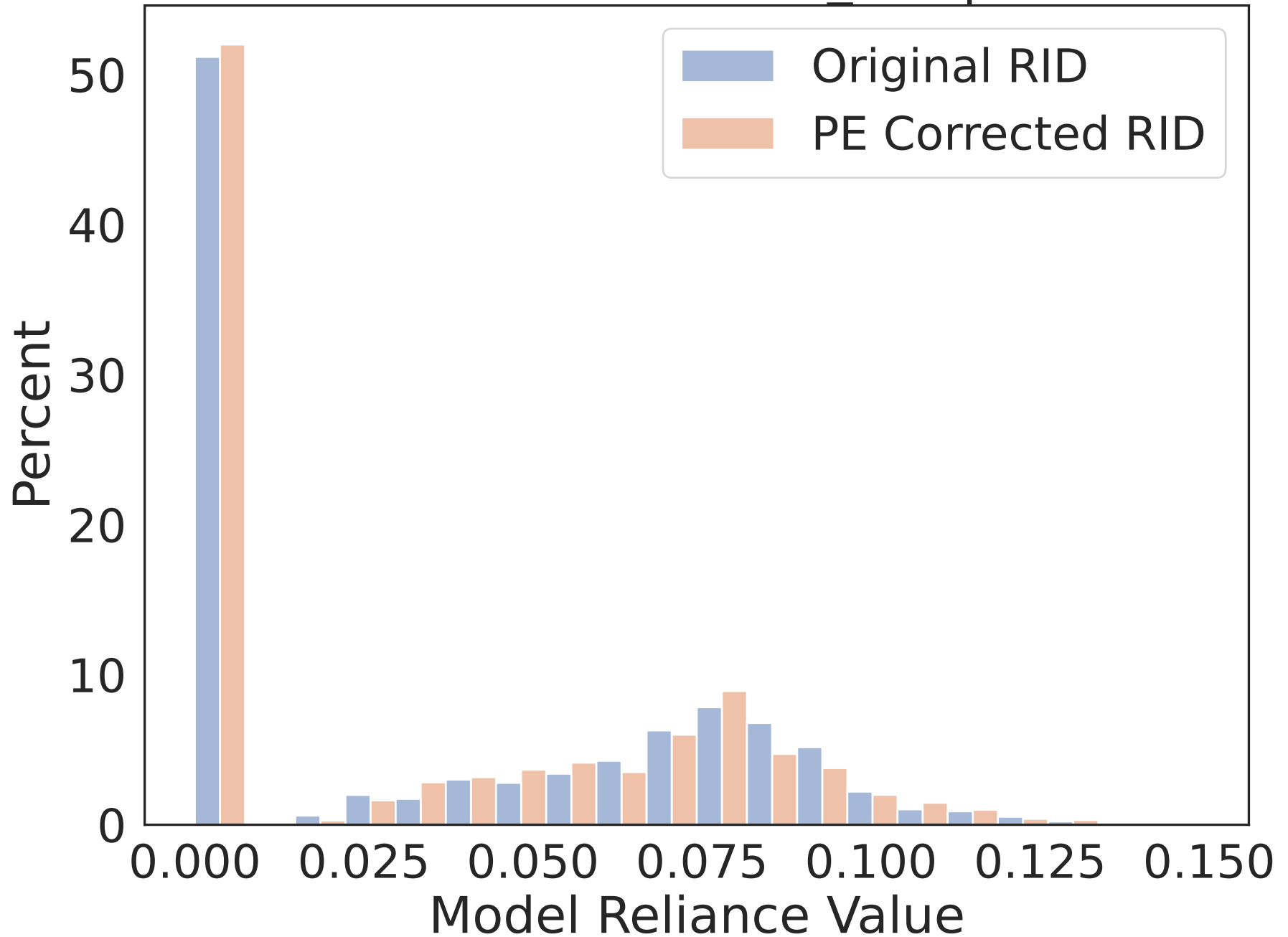
RID Distribution of Feat2_x Importance
