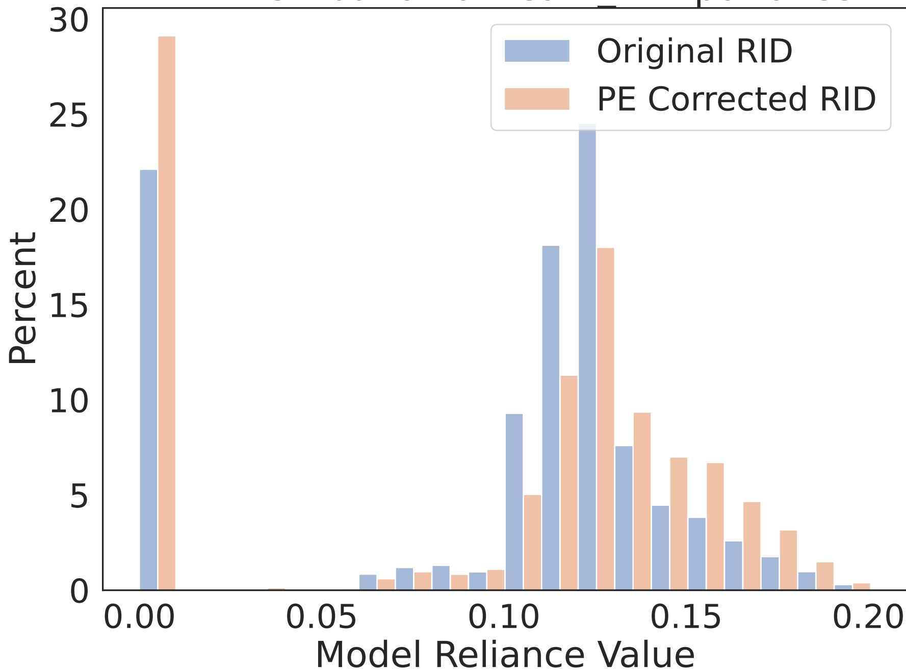
RID Distribution of Feat4_x Importance
