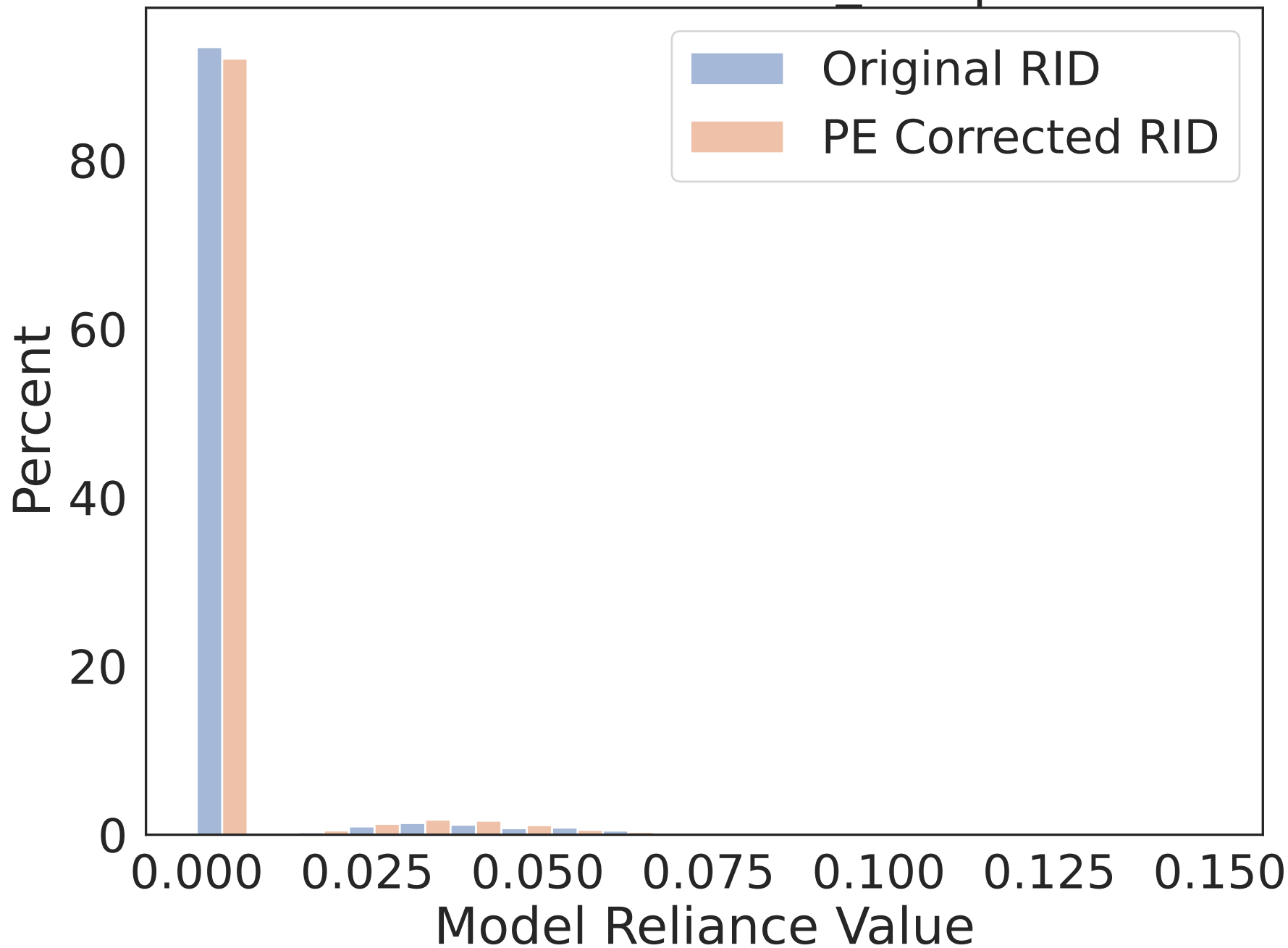
RID Distribution of Feat5_x Importance
