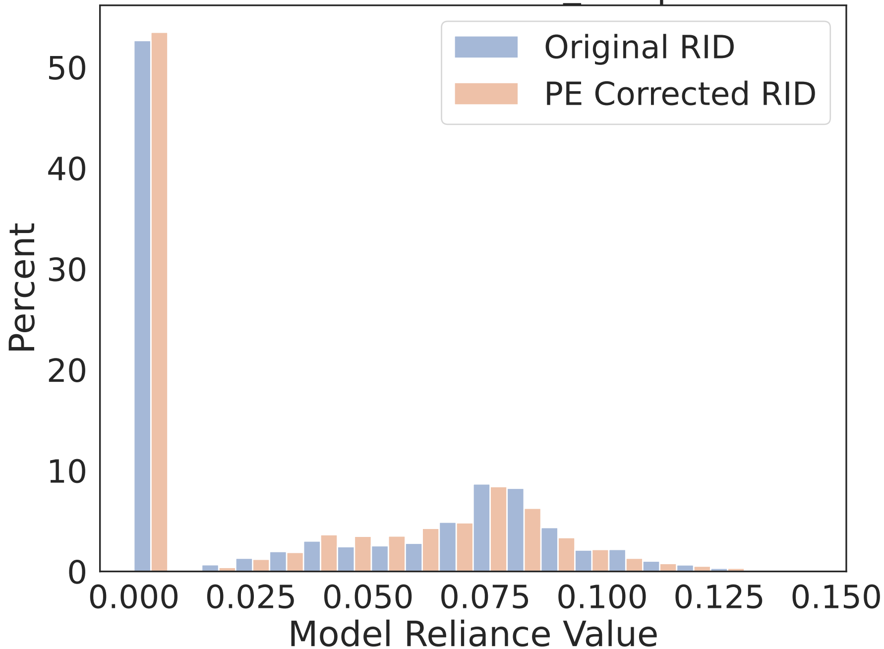
RID Distribution of Feat6_x Importance
