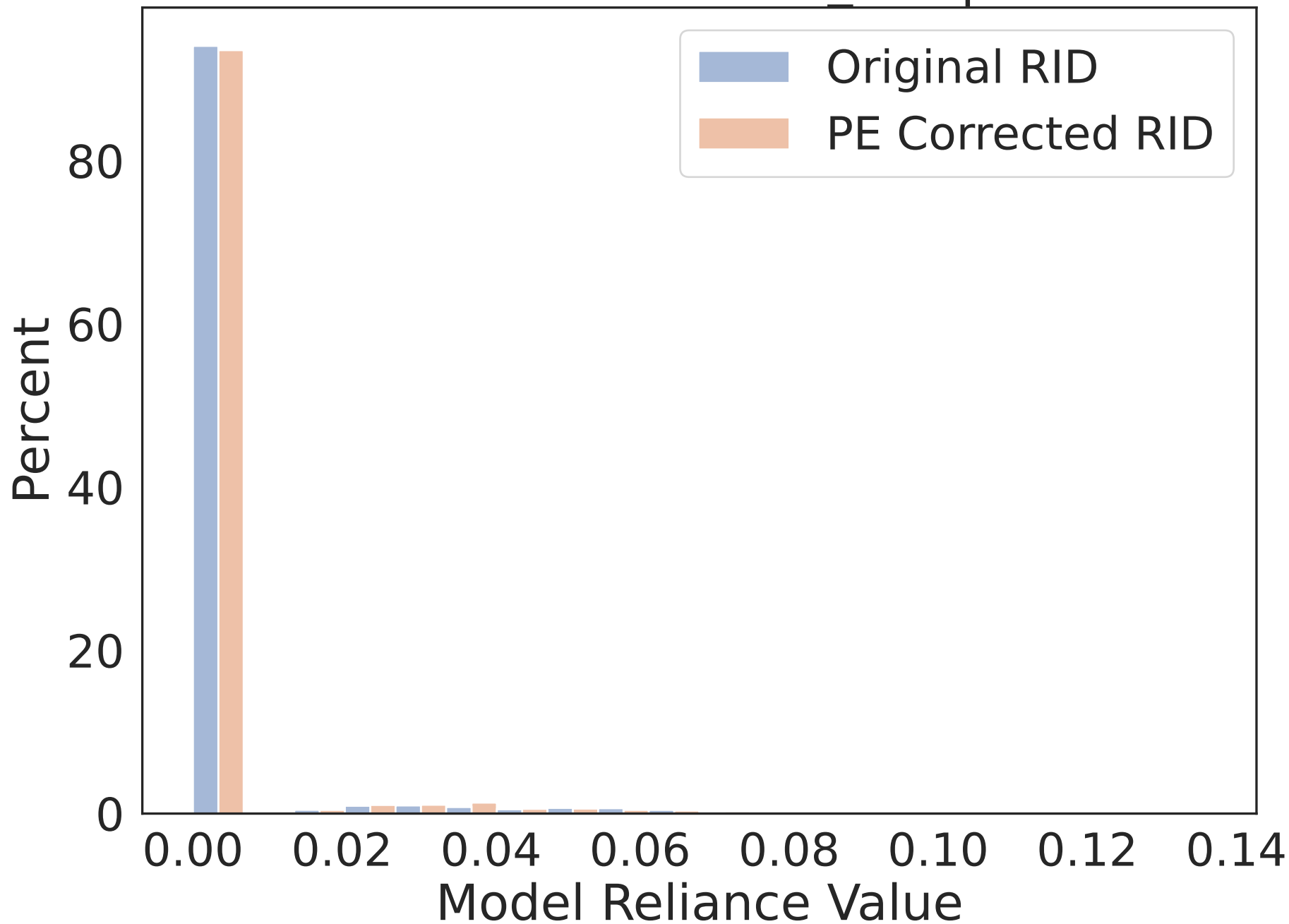
RID Distribution of Feat7_x Importance
