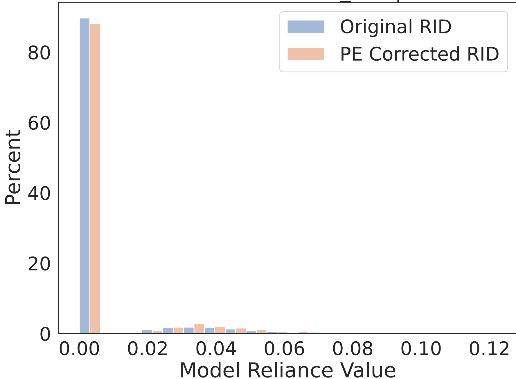
RID Distribution of Feat8_o Importance
