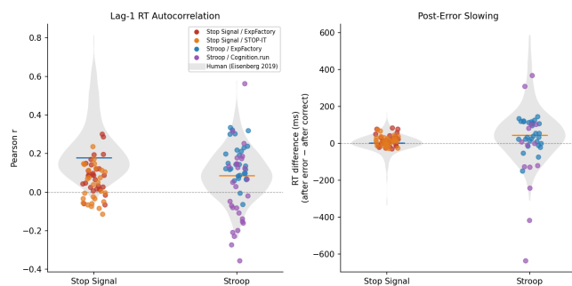
Figure 2: Sequential effects in bot and human data. Left panel: lag-1 RT autocorrelation; right panel: post-error slowing. Gray violins show the human reference distribution; colored dots represent individual bot “subjects” across task implementations.
