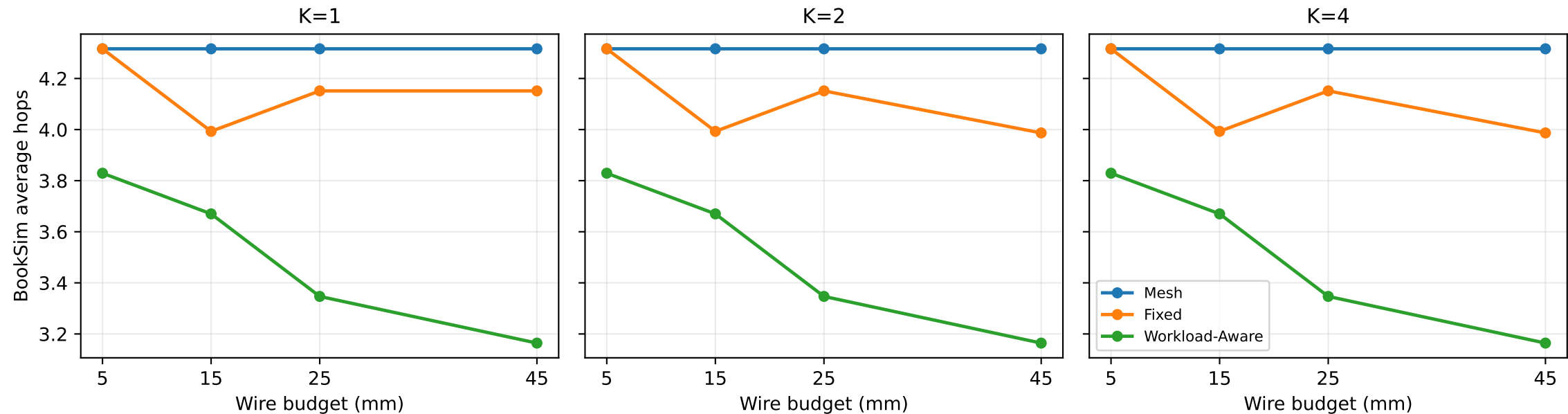
Synthetic average hops vs budget and K: transpose
