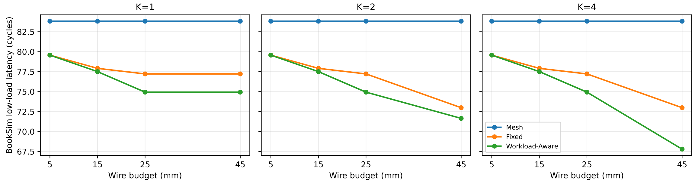
Synthetic latency vs wire budget: hotspot
