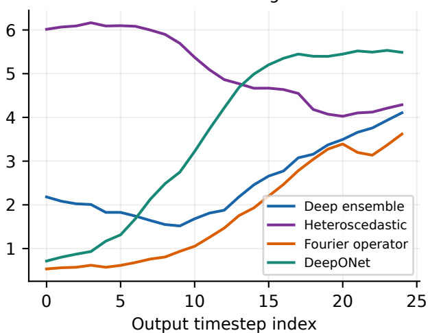
Variance shift Median full-field log RMSE
