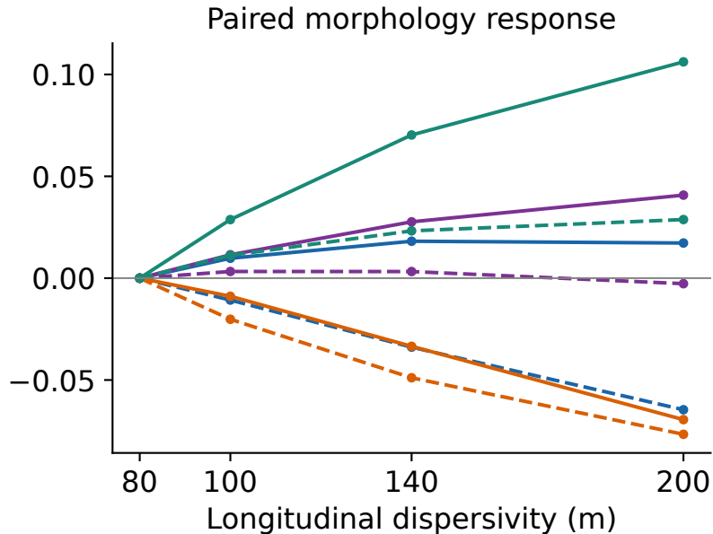
Full-field score ratio relative to 80 m
