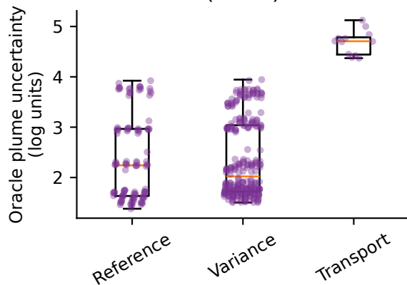
DeepONet
