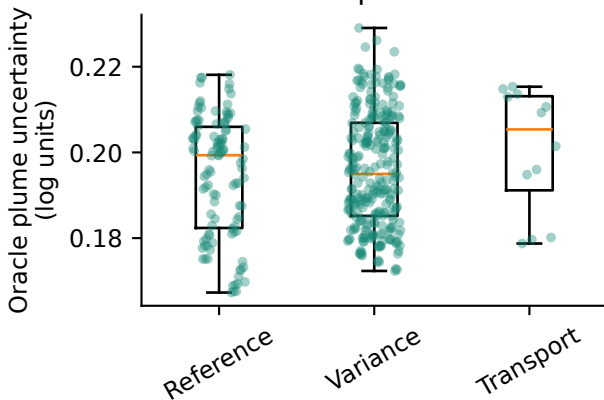
DeepONet
