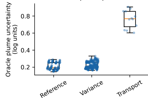
Fourier operator
