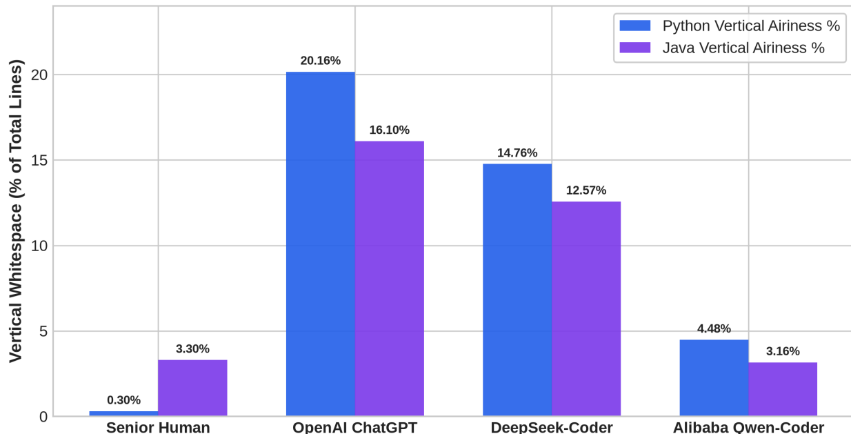
Figure 1: Vertical Whitespace Airiness ("LLM Airiness") across Human developers and AI models.
