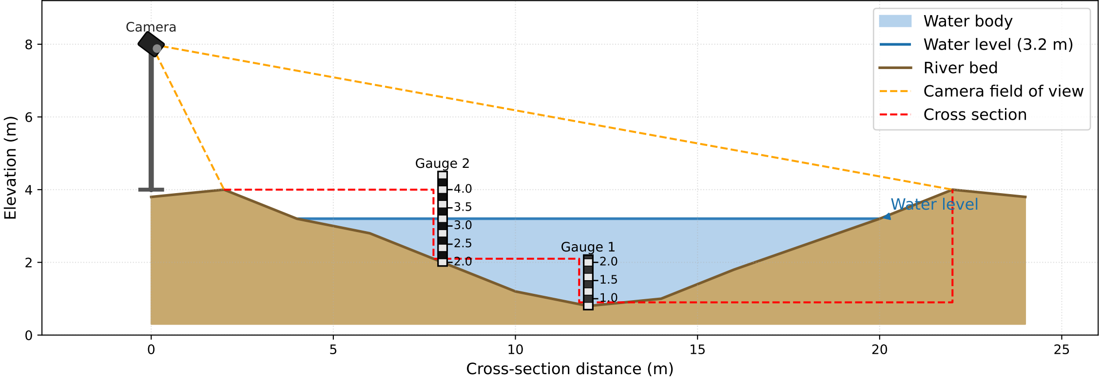
Stream cross-section: bathymetry, water level, staff gauges and camera setup
