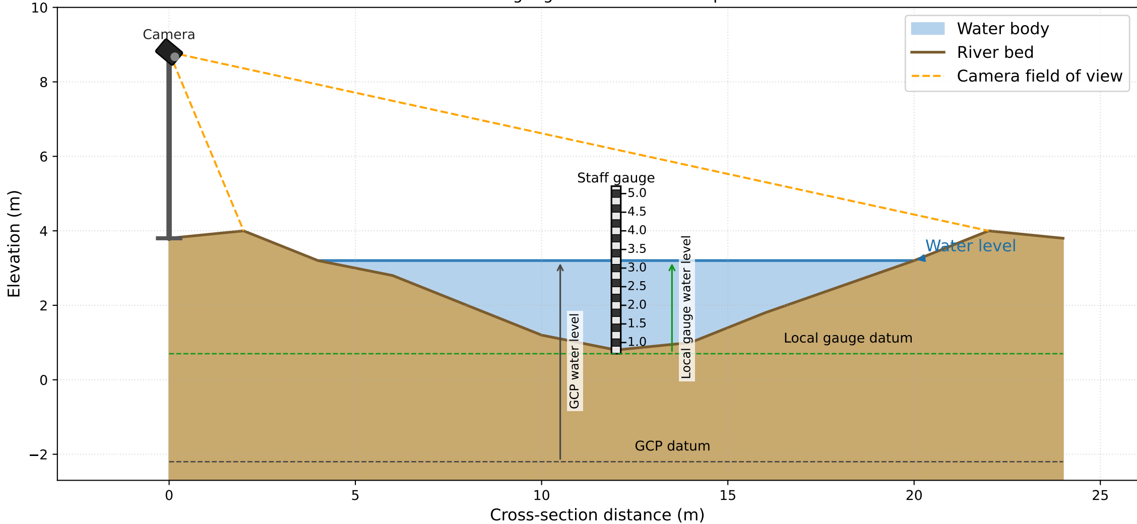
Stream cross-section: bathymetry, water level, staff gauges and camera setup
