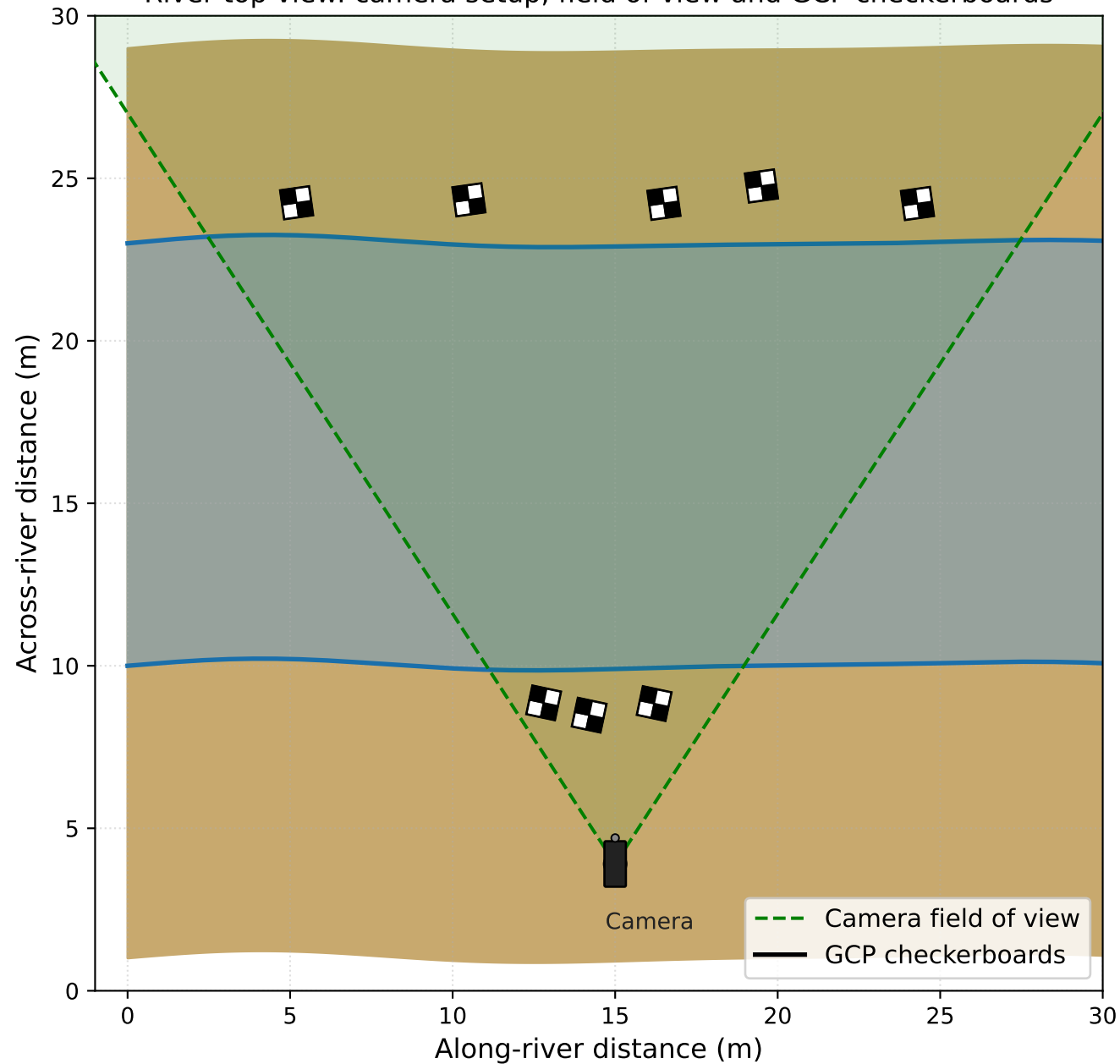
River top view: camera setup, field of view and GCP checkerboards
