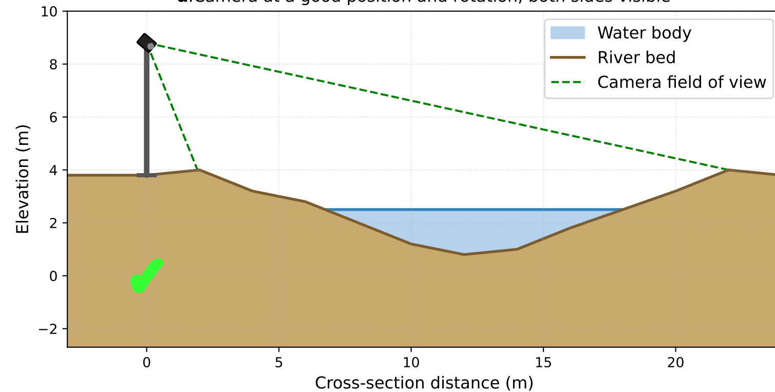
a. Camera at a good position and rotation, both sides visible
