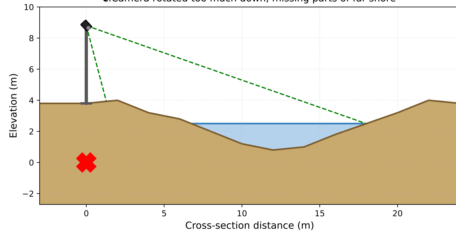
c. Camera rotated too much down, missing parts of far shore
