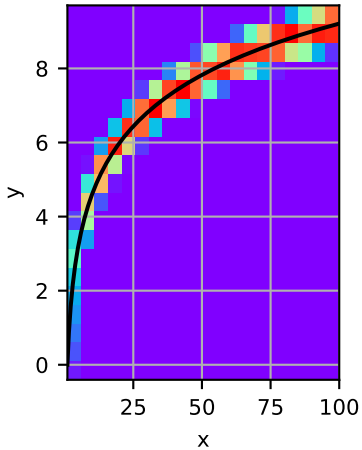
histogram2d
