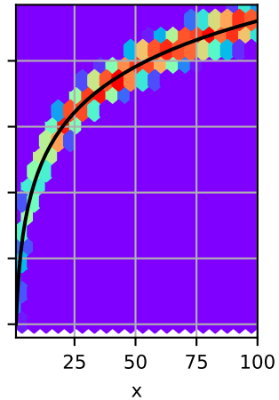
hexbin
