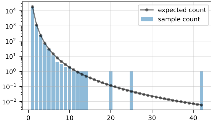
Zipf sample, a=4.0 , size=20000
