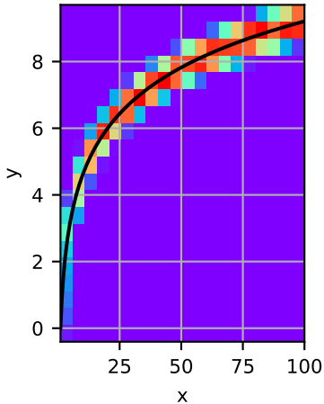
histogram2d
