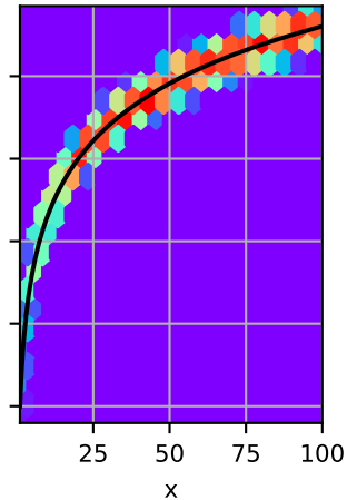
hexbin
