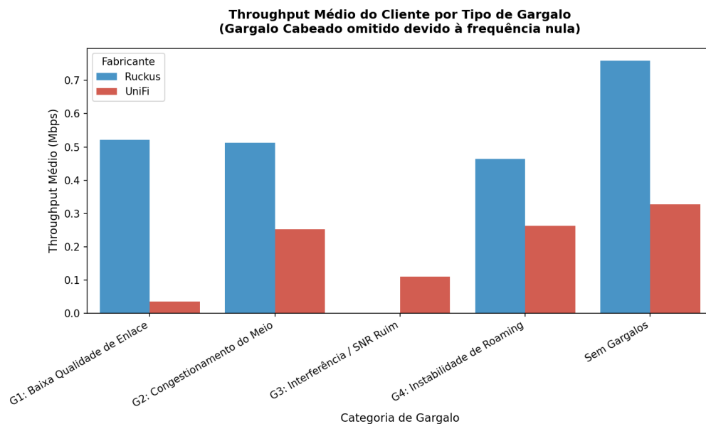
Figura 28 – Impacto no Throughput
