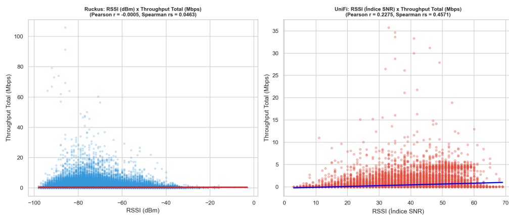
Figura 15 – RSSI x Throughput
