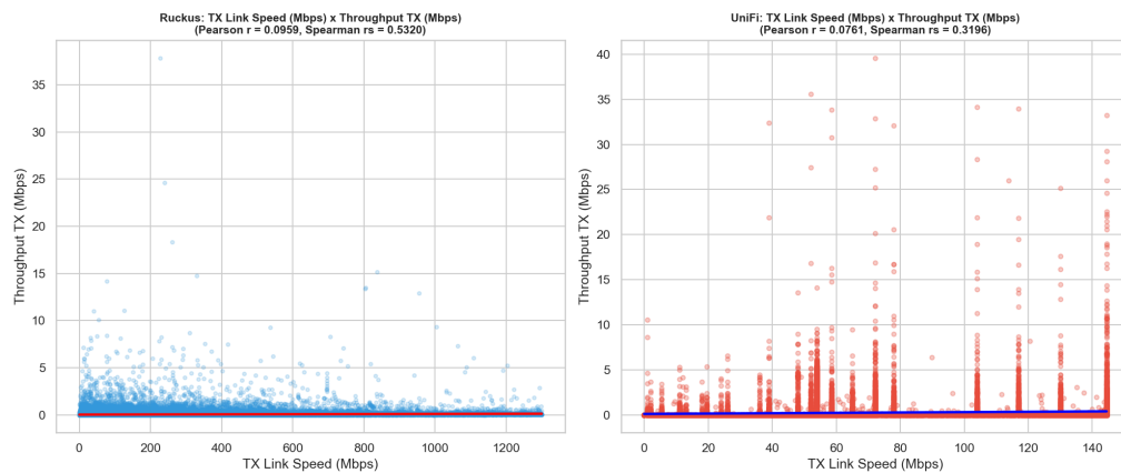
Figura 19 – Link Speed x Throughput
