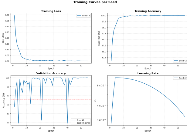
Figure 5. Training curves: (top-left) BCE loss, (top-right) training accuracy, (bottom-left) validation accuracy with the previous best baseline marked, (bottom-right) learning rate schedule.
