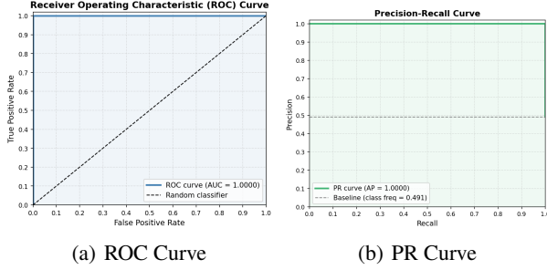
Figure 6. (a) Receiver Operating Characteristic curve with AUC score. (b) Precision-Recall curve with Average Precision score. Both are computed on the 15% held-out validation set (seed 42).
