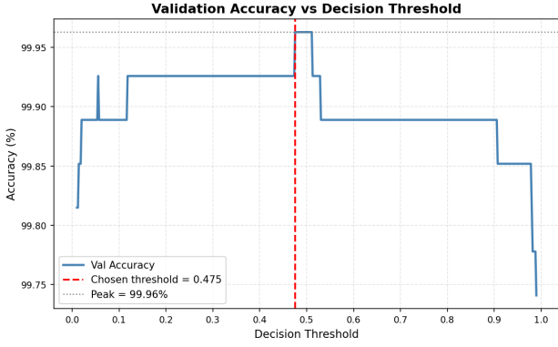
Figure 3. Validation accuracy as a function of the decision threshold. The optimal threshold (red dashed line) differs noticeably from 0.5, confirming the importance of post-hoc calibration.
