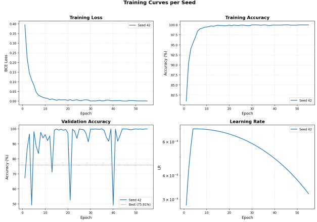
Figure 4. Training curves: (top-left) BCE loss, (top-right) training accuracy, (bottom-left) validation accuracy with the previous best baseline marked, (bottom-right) learning rate schedule.
