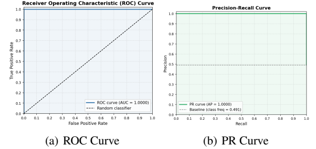
Figure 5. (a) Receiver Operating Characteristic curve with AUC score. (b) Precision-Recall curve with Average Precision score. Both are computed on the 15% held-out validation set (seed 42).
