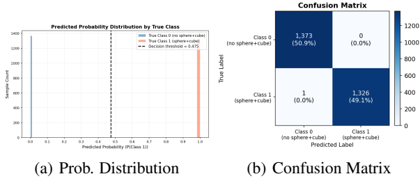
Figure 6. (a) Predicted probability histogram by true class. A clear bimodal separation is visible, with the decision threshold marked. (b) Confusion matrix on the validation set.
