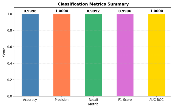
Figure 7. Classification metrics on the held-out validation set (Accuracy, Precision, Recall, F1-Score, AUC-ROC).
