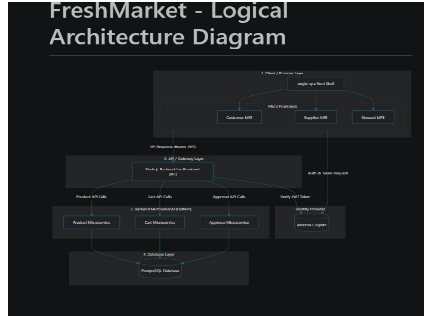
Logical Architecture Diagram ( single-spa - Node.js BFF - FastAPI Microservices -PostgreSQL )
