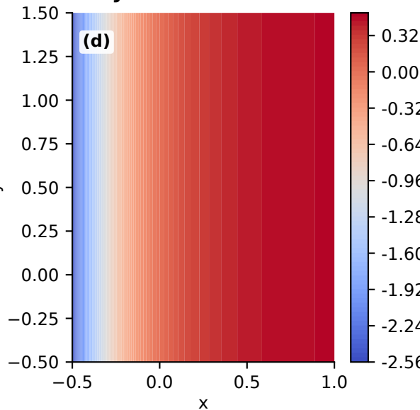
Analytical Pressure Field
