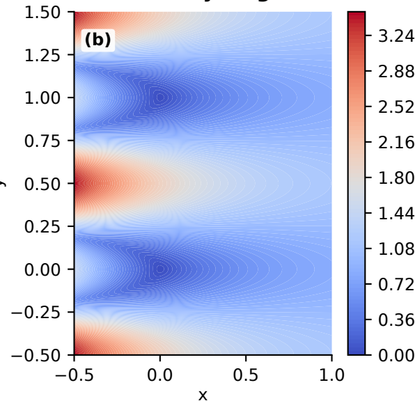
PINN Pressure Field
