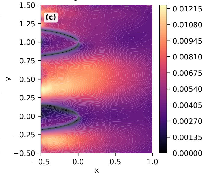
Pressure Absolute Error
