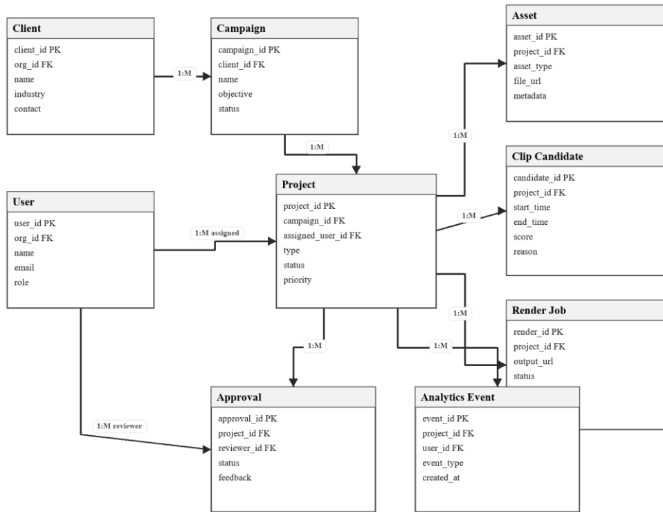
ContentFlow AI Entity Relationship Diagram
