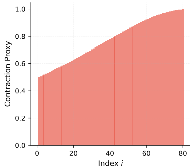
Inference Difficulty
