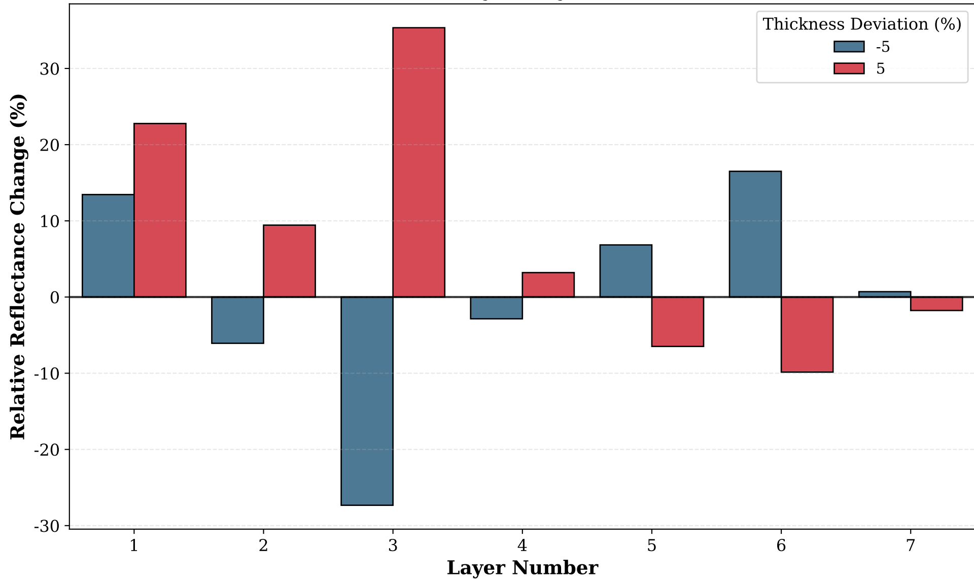
Thickness Sensitivity Analysis ( \pm 5\% Deviation)
