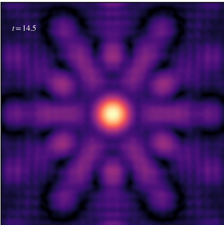
(a) fusion ( k_0=0.5 )
