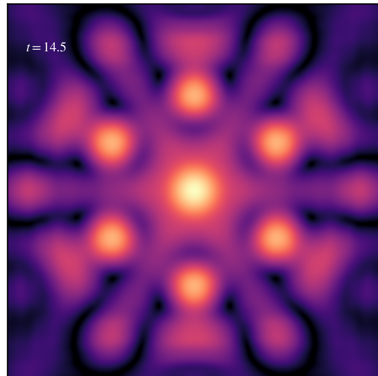
(b) fragmentation ( k_0=0.0 )
