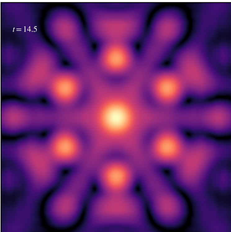
(c) transition ( k_0=0.1 )
